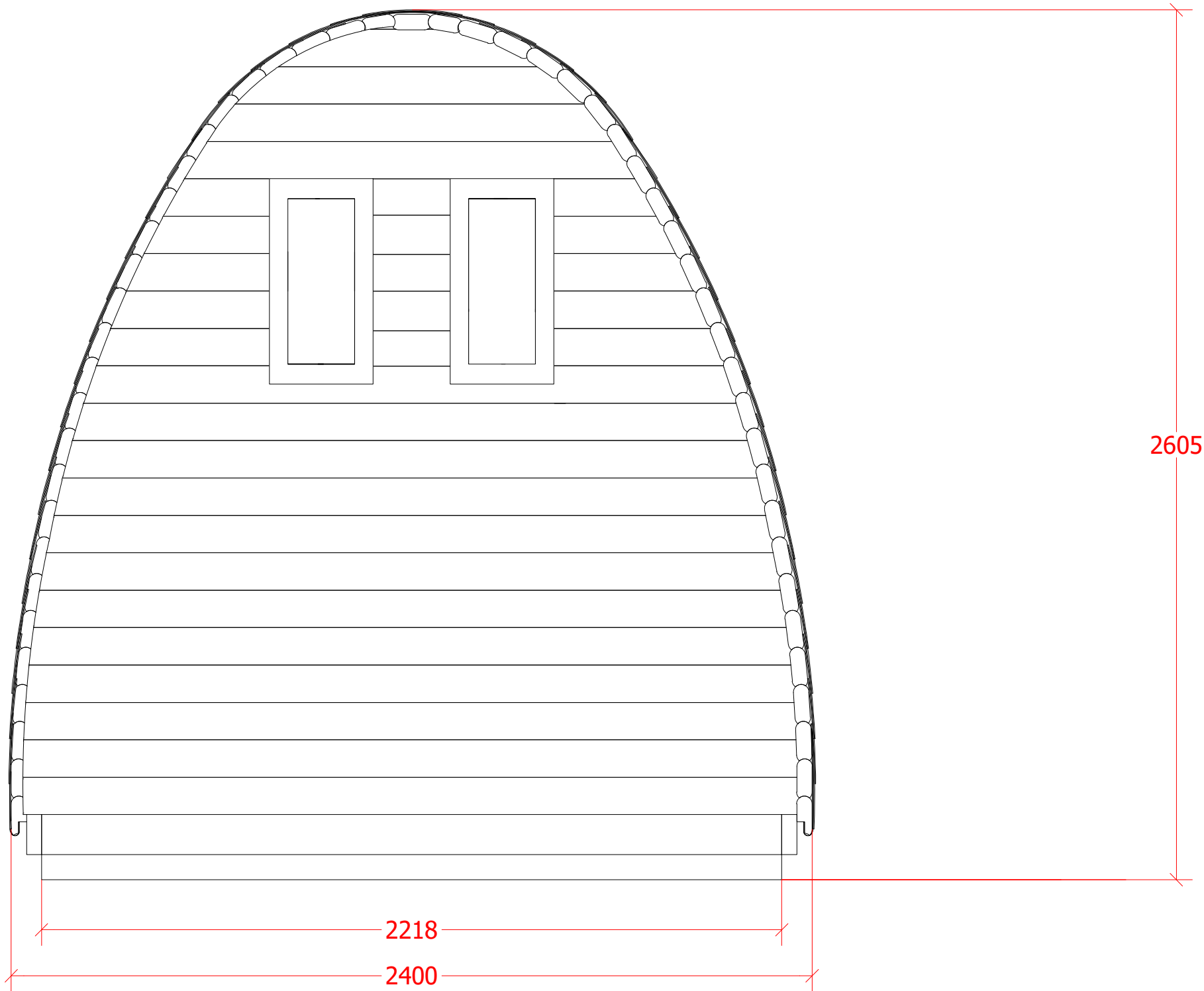
Back ( 1 :15 )
