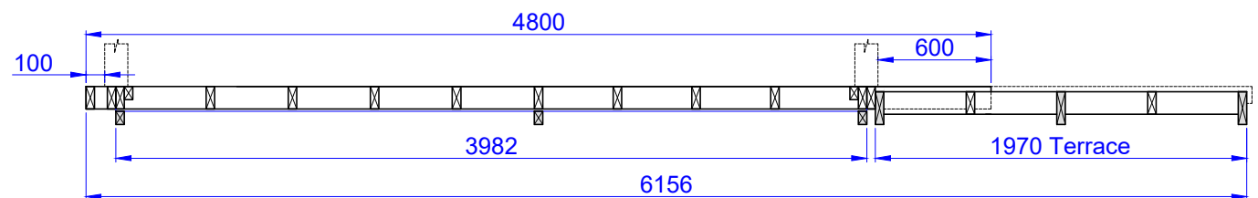
Cut view
