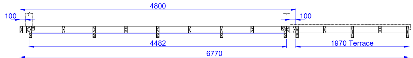
Cut view
