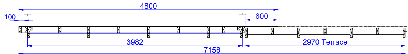
Cut view
