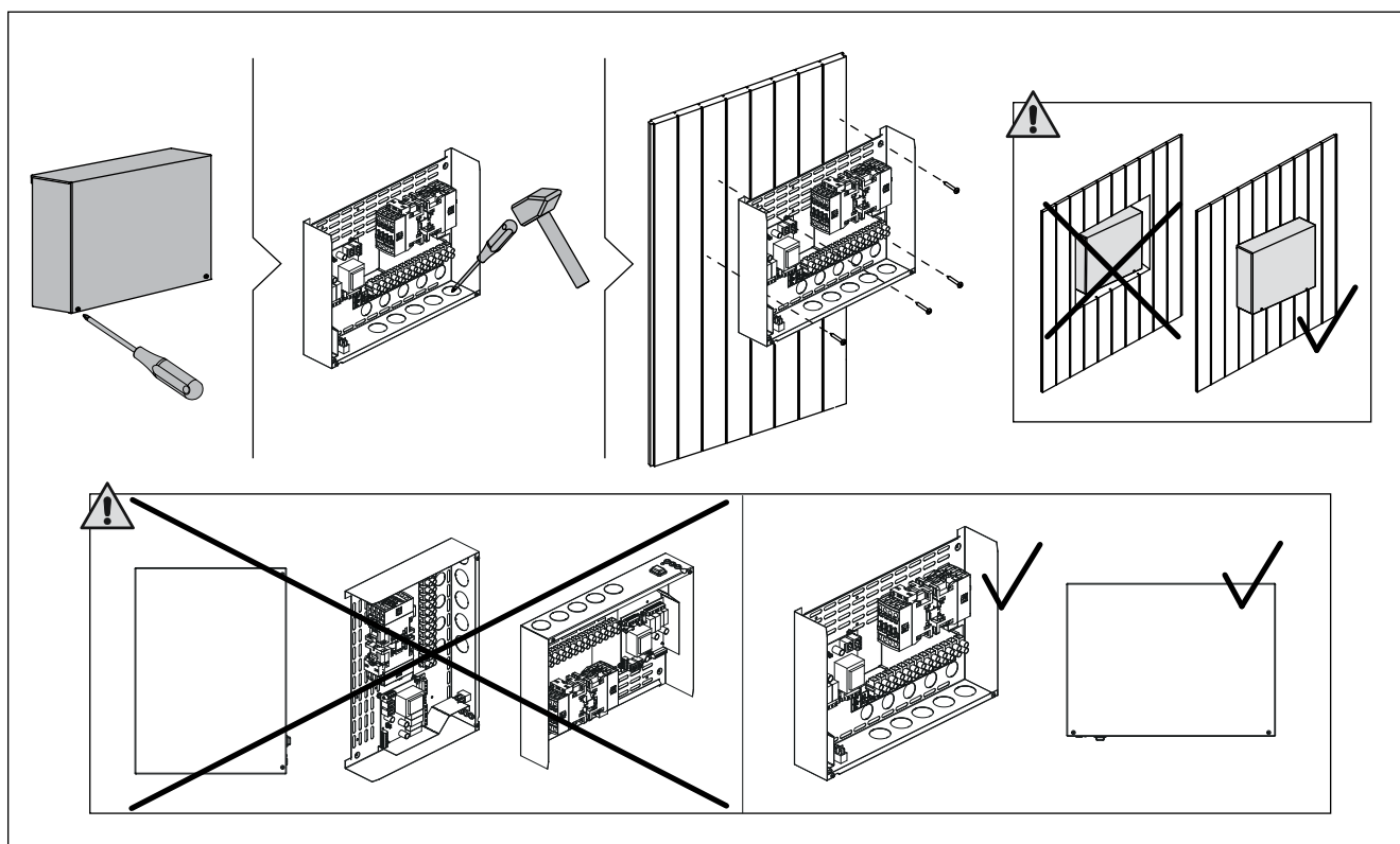
Figure 5a. Opening the power unit cover and mounting the unit to a wall
